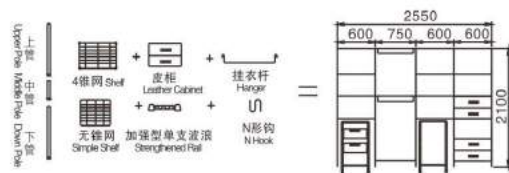
品名：衣柜收纳组合1 Name: Clothes Closet Units 1
