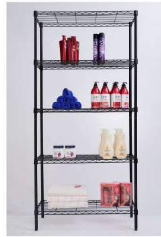
型号:CJ-B1256 Item No.:CJ-B1256 名称:五层环氧置物架(碳灰色) Name:5 Tier Epoxy Wire Shelving 产品尺寸: L900xW350xH1800(mm) Product Dimension: L900xW350xH1800(mm)
