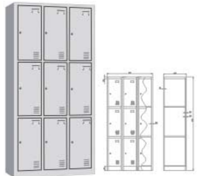
JF-3B3A H1850 × W900 × D450mm
