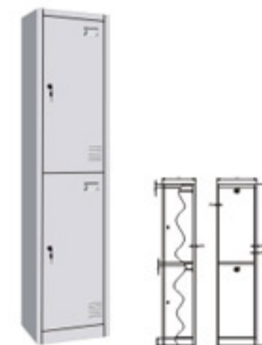
JF-1B2A H1850 × W380 × D450mm
