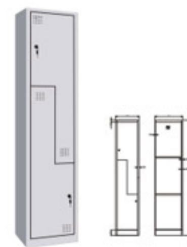
JF-Z001 H1850 × W400 × D450mm
