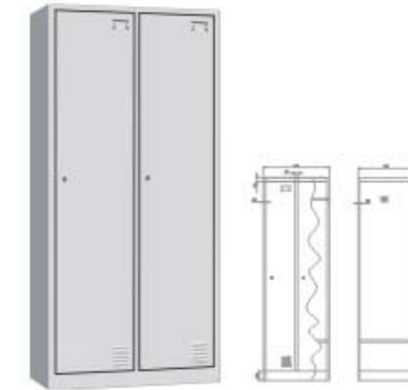
JF-2B1A H1850 × W900 × D450mm
